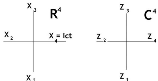
FIG. 3. In \mathbb{C}^4 SQS, there is no temporal dimension.
