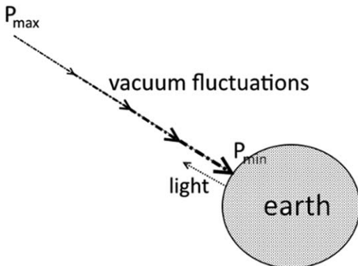
FIG. 2. The redshift of light moving from the Earth's surface upwards.
