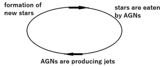
FIG. 5. Energy circulation in the universe is permanent.
