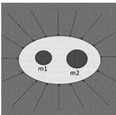
FIG. 4. Gravity for acts from outer space toward the center of physical objects.
