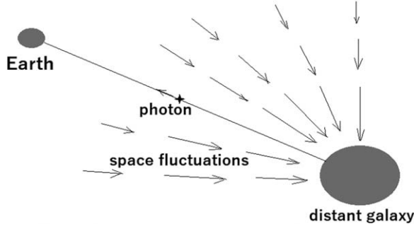
FIG. 1. Light is losing some of its energy when moving in the opposite direction of the space fluctuations that carry gravity.
